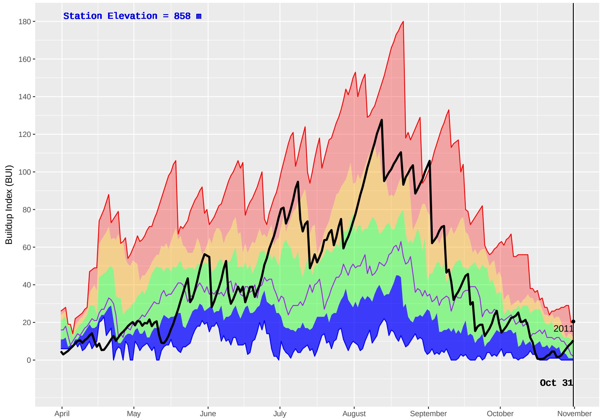
BEDNESTI (175) : Historical (1993–2016) and Current (2017) Noon Buildup Index (BUI)
