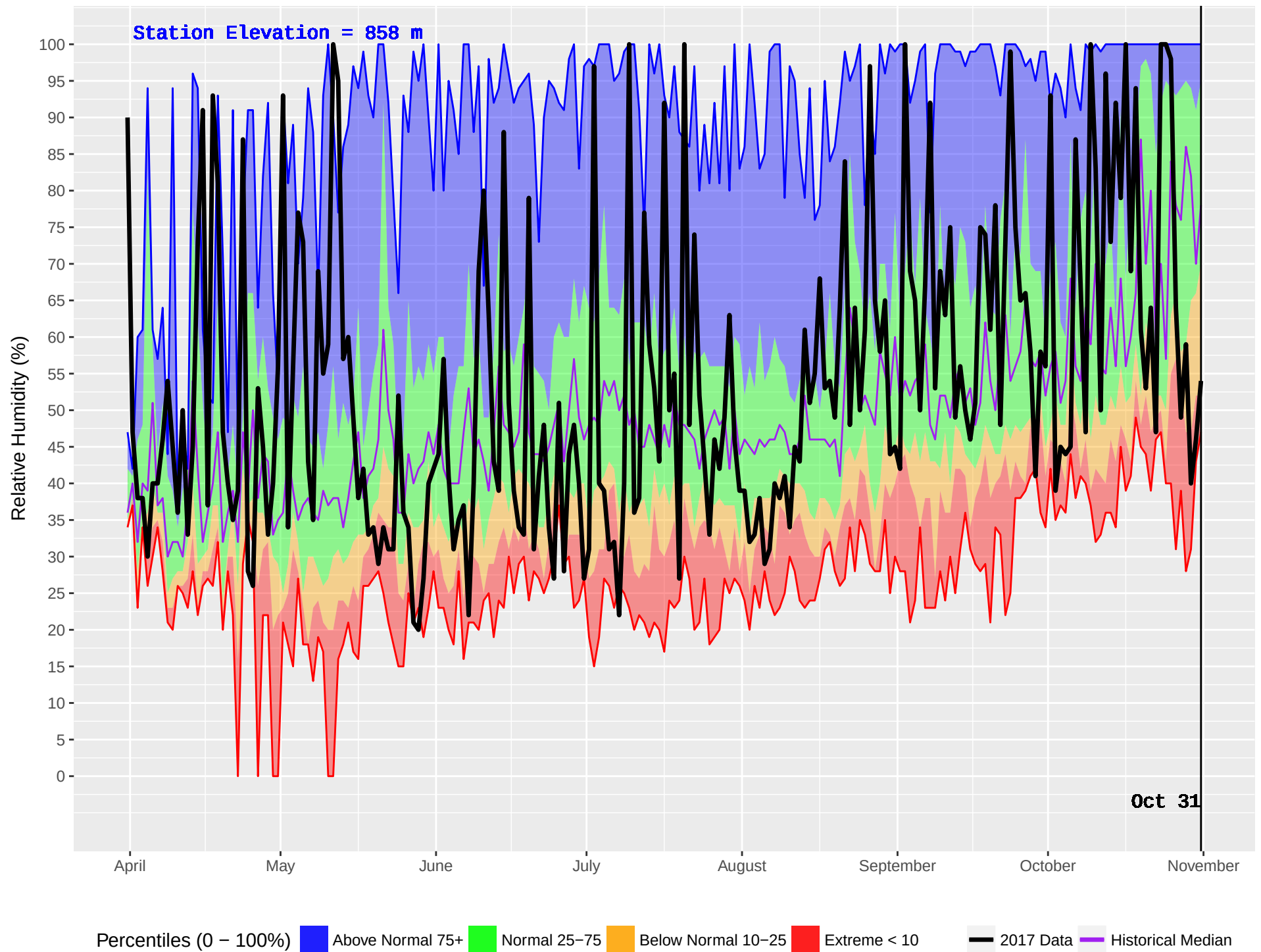
BEDNESTI (175) : Historical (1993–2016) and Current (2017) Noon Relative Humidity
