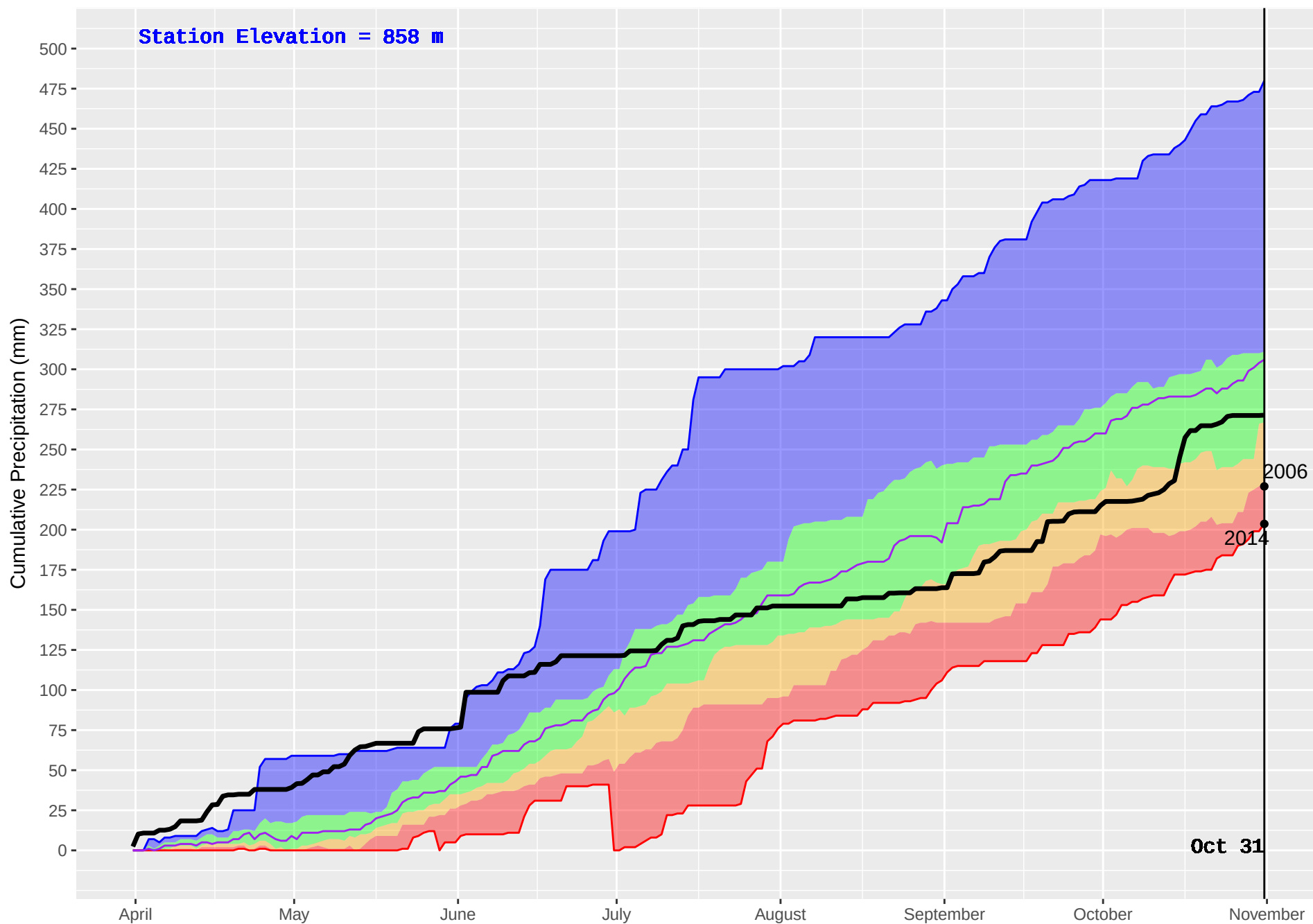
BEDNESTI (175) : Historical (1993–2016) and Current (2017) Noon Cumulative Precipitation
