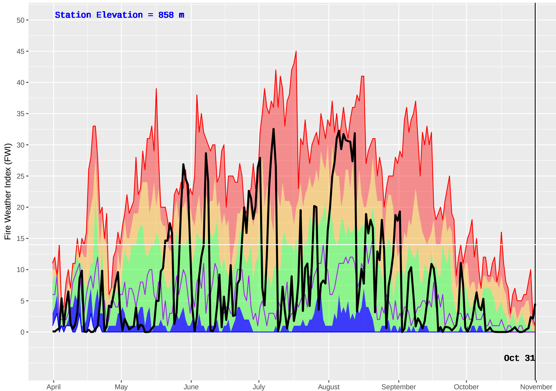
BEDNESTI (175) : Historical (1993–2016) and Current (2017) Noon Fire Weather Index (FWI)
