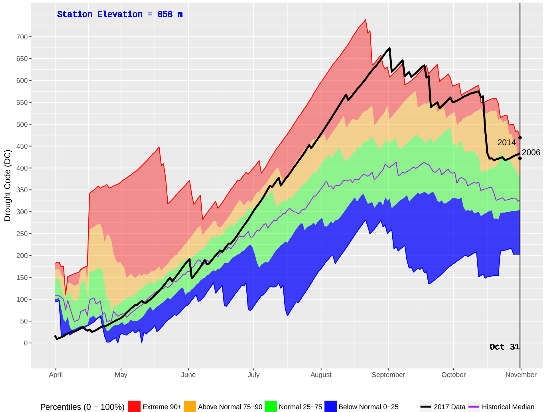
BEDNESTI (175) : Historical (1993–2016) and Current (2017) Noon Drought Code (DC)
