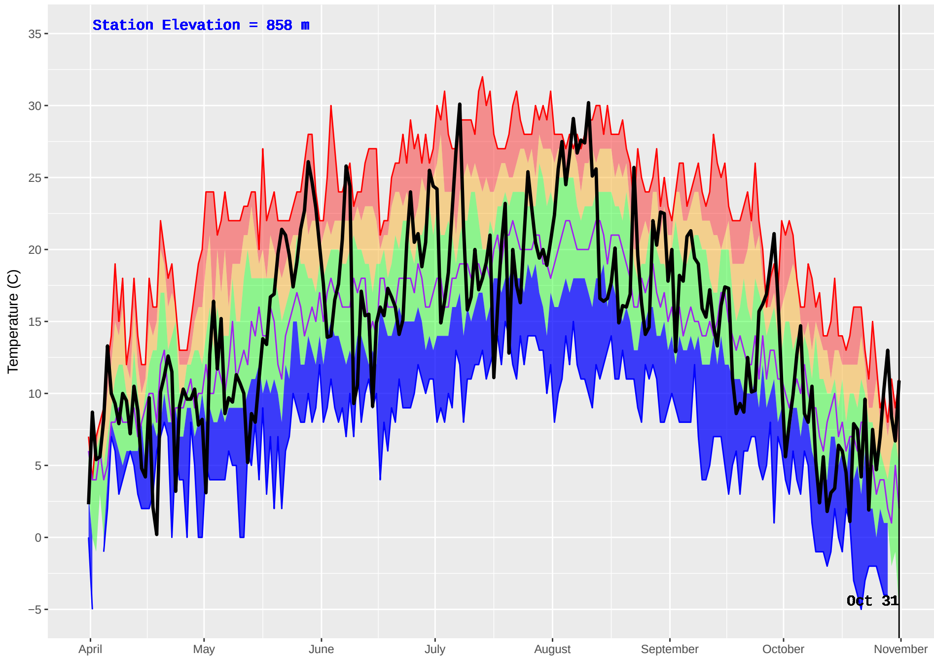
BEDNESTI (175) : Historical (1993–2016) and Current (2017) Noon Temperature
